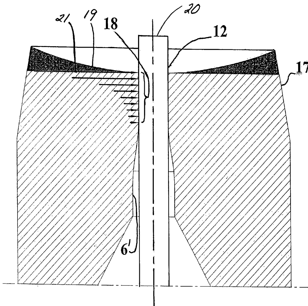
Fig. 10 (Prior art)
