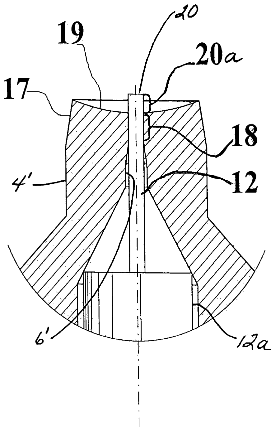
Fig. 8 (Prior art)
